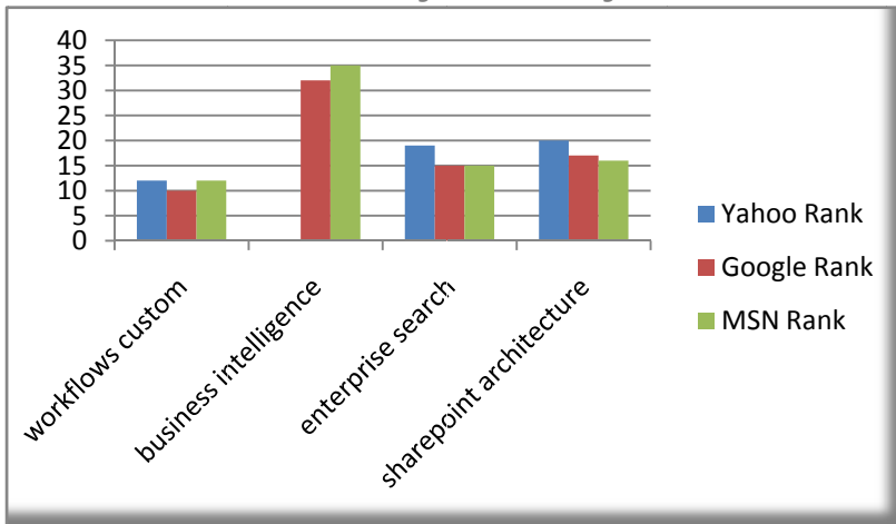
Keyword Analysis
