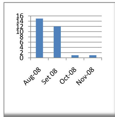
Broken Links
